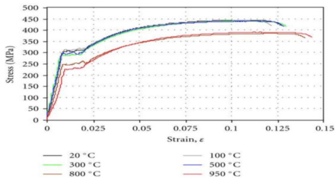
Figure 2. Graph of the Stress and Strain Relationship
