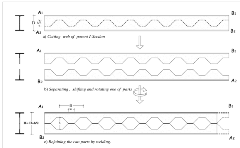
Figure 1. Making Castellated Beam Hexagon Shape
